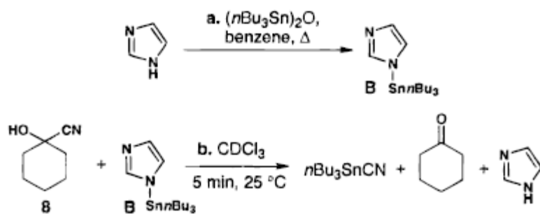
Scheme 3. Evidence for the Participation of Intermediate B in the Regeneration of Ketones from Cyanohydrins
